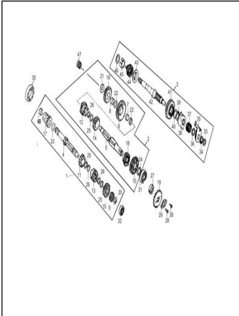
FIGURA N° 10: TRANSMISION (1/2)
