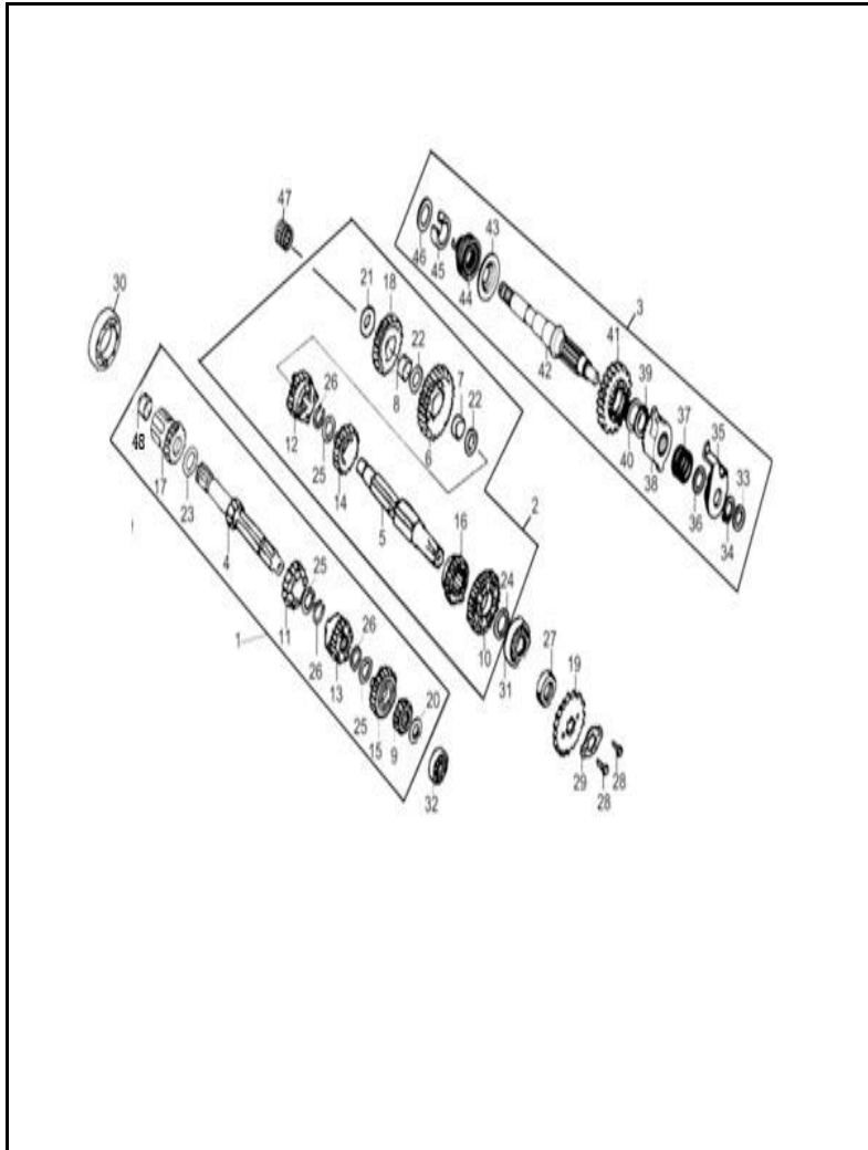
FIGURA N° 10: TRANSMISION (2/2)
